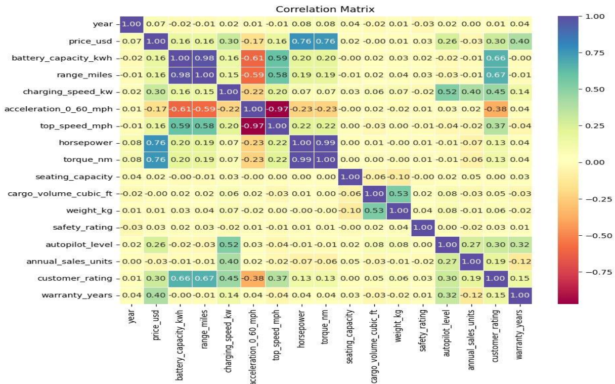
Figure 5: Correlation Matrix — All Numeric Features
